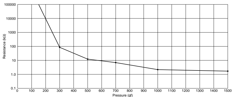
Pressure vs Resistance (average from 3 samples)
